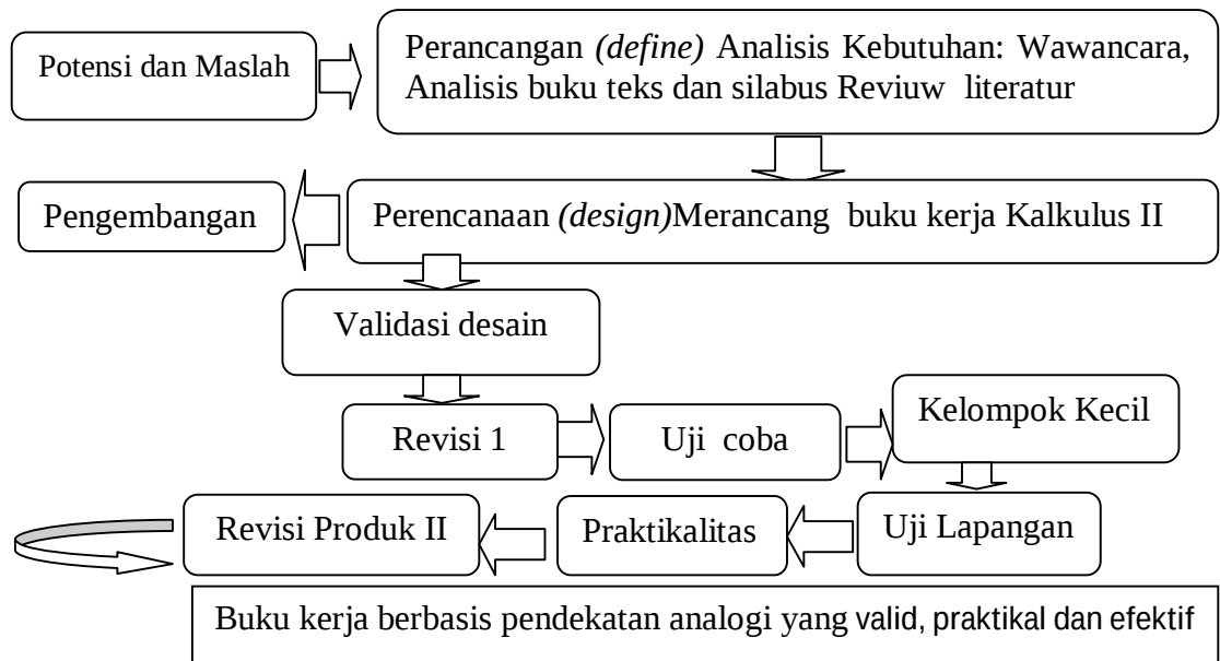
Gambar 1. Prosedur Penelitian
